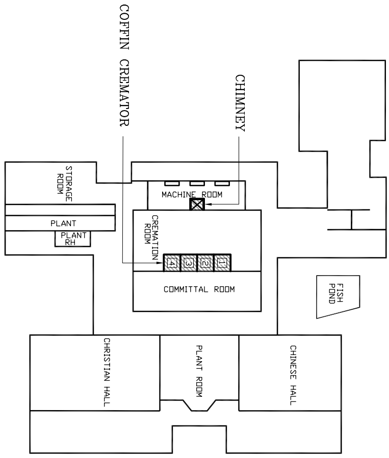
PLAN VIEW OF COFFIN CREMATORIUM (G/F)
